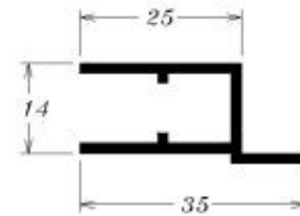
Y-106 0.335 kg/m
