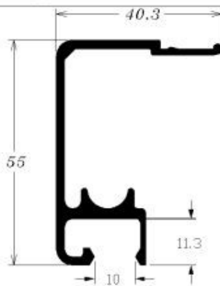
AL-60 0.863 kg/m
