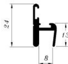
AL-47 0.272 kg/m
